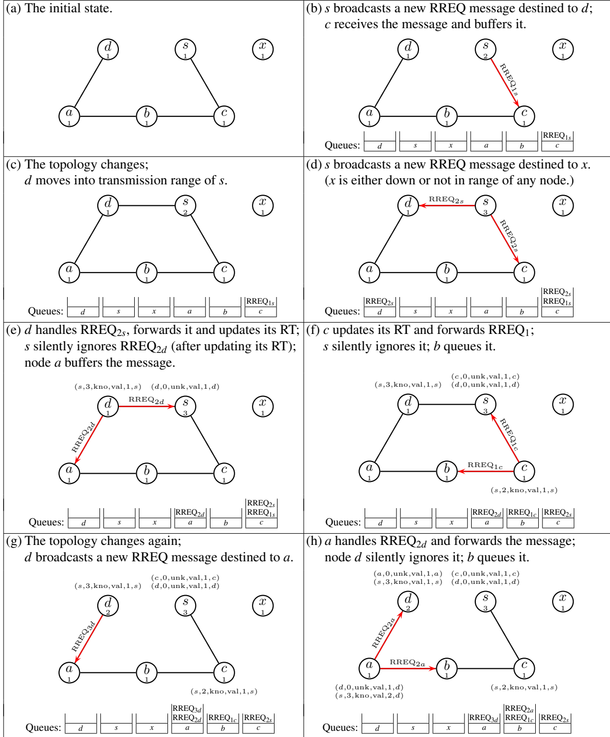
Figure 9: Self-entries
