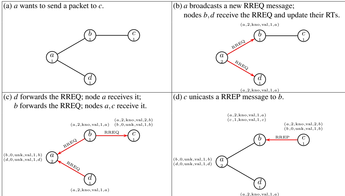
Figure 2: Simple example
