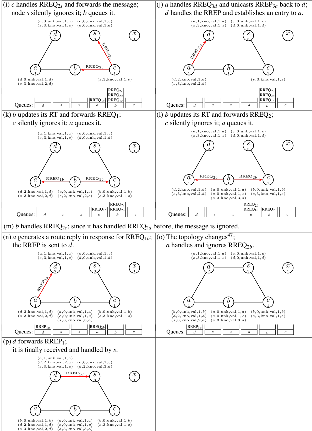
Figure 9 (cont'd): Self-entries
