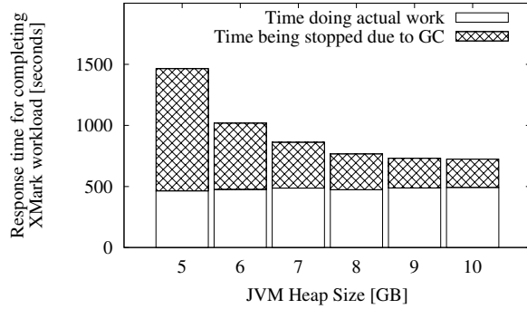
Figure 2. Response time vs. JVM heap size
