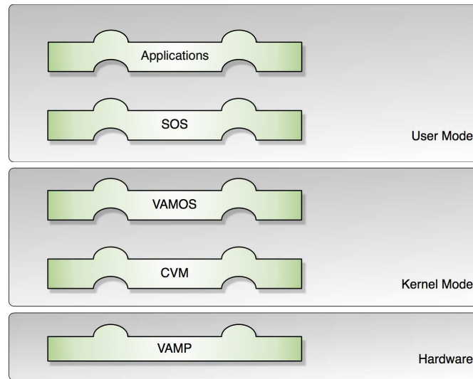
Fig. 8. Verisoft: system layers.
